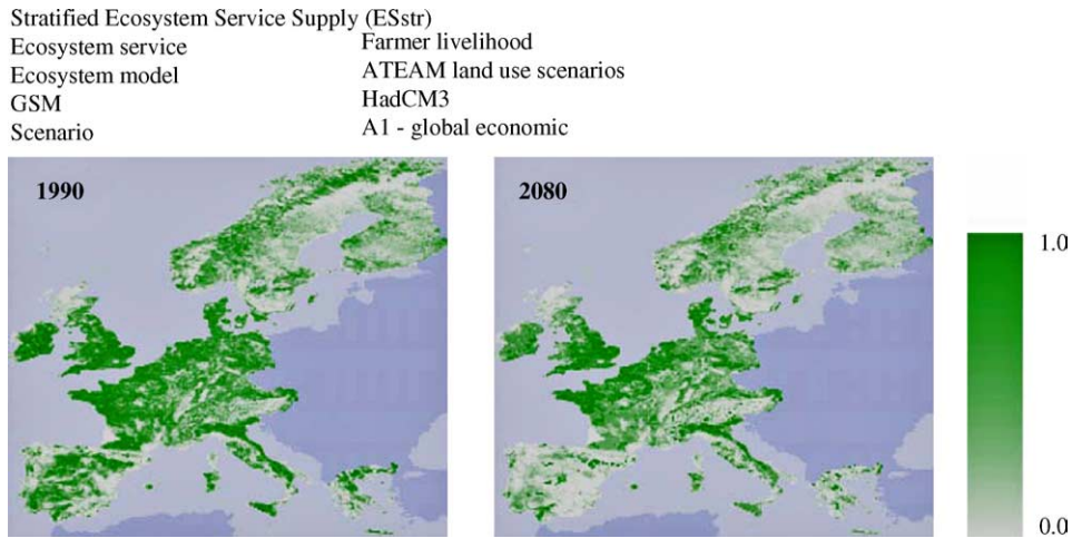
Fig. 4. Stratified ecosystem service supply for the ecosystem service indicator ‘farmer livelihood’. The ecosystem service supply maps for ‘farmer livelihood’ (Fig. 1) are stratified by the environmental strata (Fig. 3).
