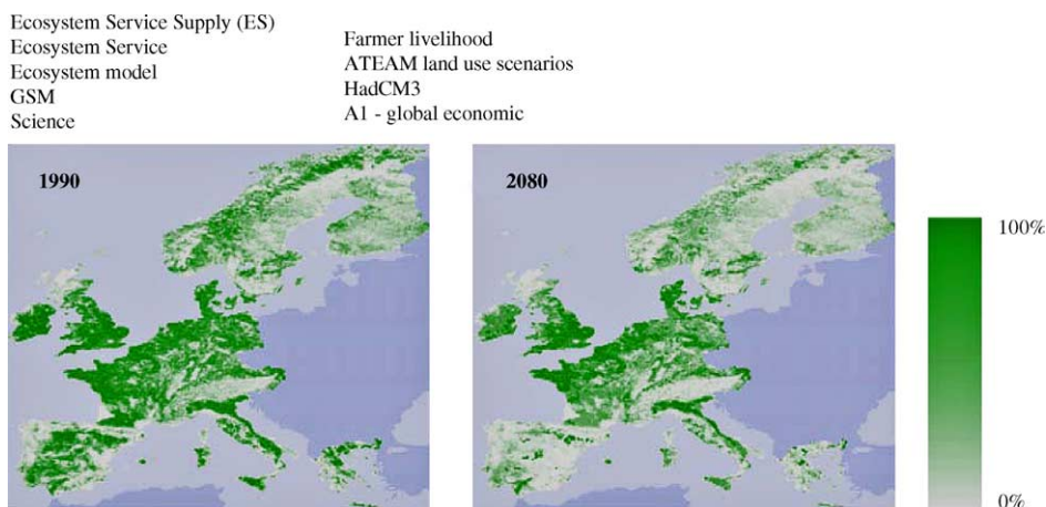
Fig. 2. Ecosystem service supply indicator for ‘farmer livelihood’, as modelled by the ATEAM land use scenarios for baseline conditions and the A1 scenario for the 2080 time slice.
