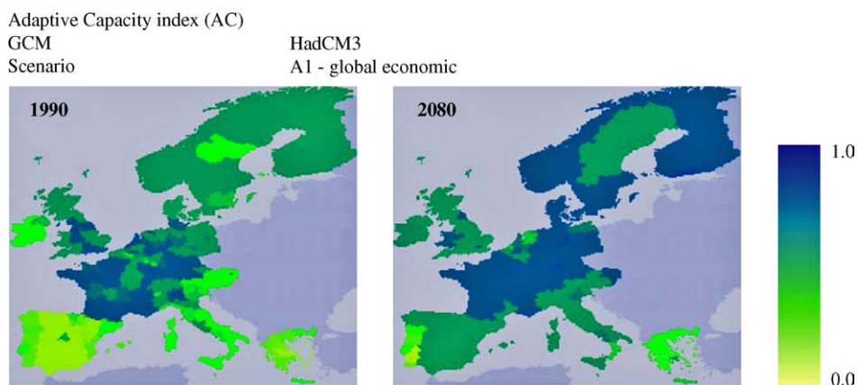
Fig. 6. Socio-economic indicators have been aggregated to a generic adaptive capacity index. Trends in the original indicators were linked to the SRES scenarios in order to map adaptive capacity in the 21st century.
