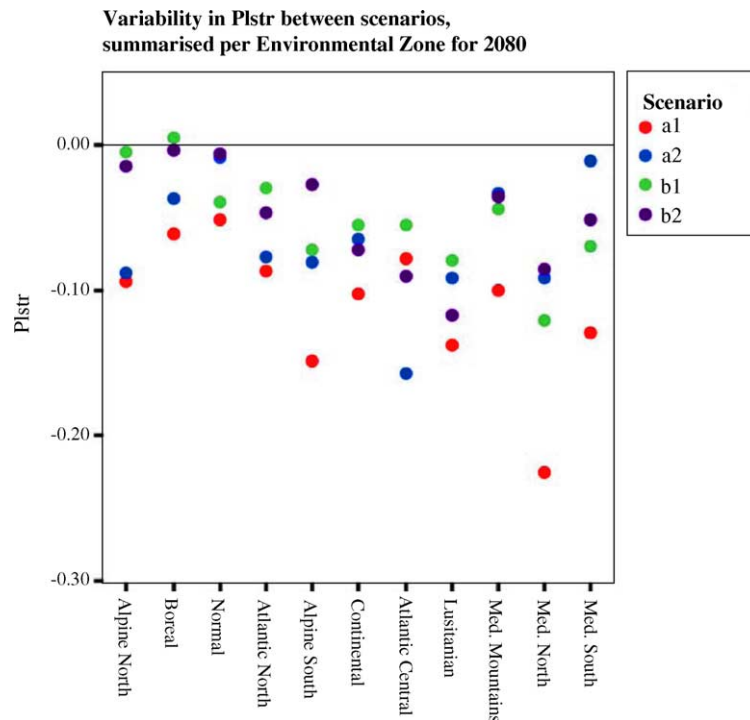
Fig. 9. Summary of mean stratified potential impacts (Plstr) for different environmental zones. These summary plots help in analysing the impacts of multiple scenarios in different regions.
