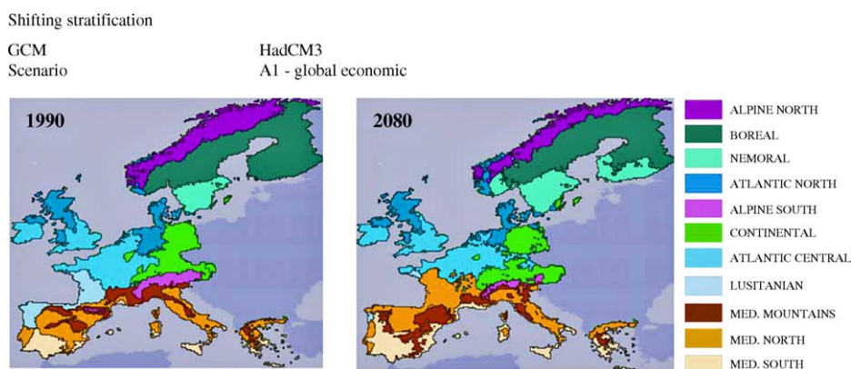
Fig. 3. Environmental Stratification of Europe (EnS), in 84 strata, here aggregated to environmental zones for presentation purposes.
