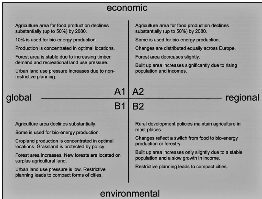
Fig. 1. Summary of the main trends in the ATEAM land use scenarios (Rounsevell et al., 2005), following the IPCC SRES scenarios (Nakicenovic et al., 2000).
