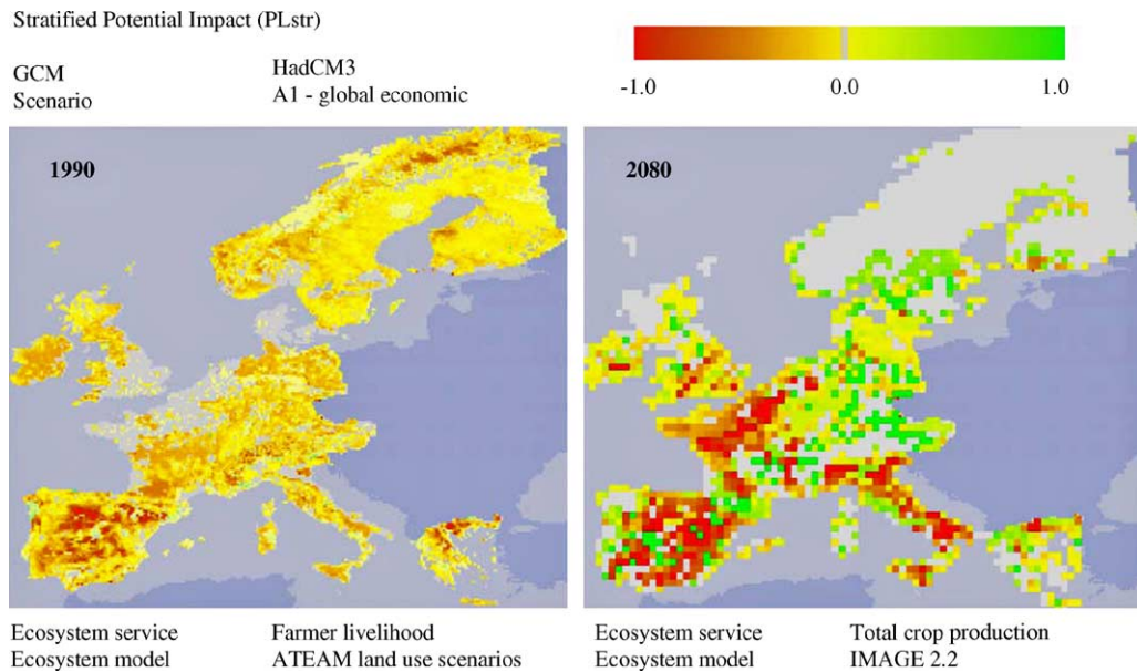
Fig. 12. Maps of changing potential impacts for the ecosystem services 'farmer livelihood' (10 arcmin resolution) and 'total crop production' (0.5° resolution). Because both maps were created using the same stratification, they can be compared.
