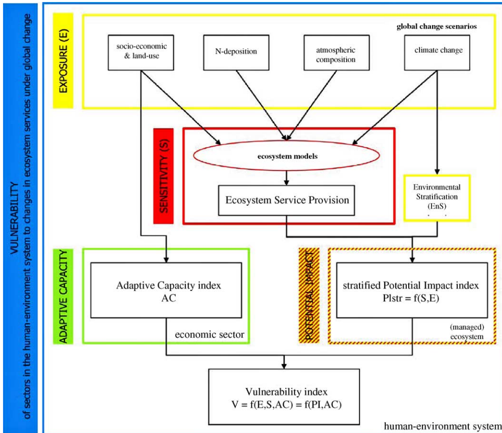
Fig. 7. Summary of the ATEAM approach to quantify vulnerability. Global change scenarios of exposure are the drivers of a suite of ecosystem models that make projections for future ecosystem services supply for a 10 arcmin × 10 arcmin spatial grid of Europe. The social-economic scenarios are used to project developments in macro-scale adaptive capacity. The climate change scenarios are used to create a scheme for stratifying of potential impacts supply to a regional environmental context. Changes in the stratified ecosystem service supply compared to baseline conditions reflect the changing potential impact of a given location. The changes in potential impact and adaptive capacity indices can be combined, at least visually, to create European maps of regional vulnerability.
