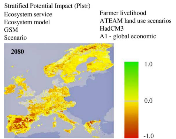
Fig. 5. Stratified potential impact for the ecosystem service indicator Farmer livelihood . Positive values indicate an increase of ecosystem service provision relative to environmental conditions, and therefore a positive potential impact, while negative potential impacts are the result of a relative decrease in ecosystem service provision compared to 1990.
